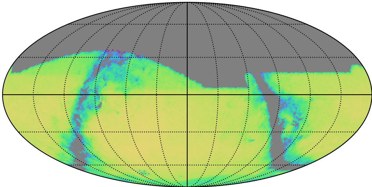
roman_v3.3_10yrs g band and non-DD: QSONumberCountsMetric
