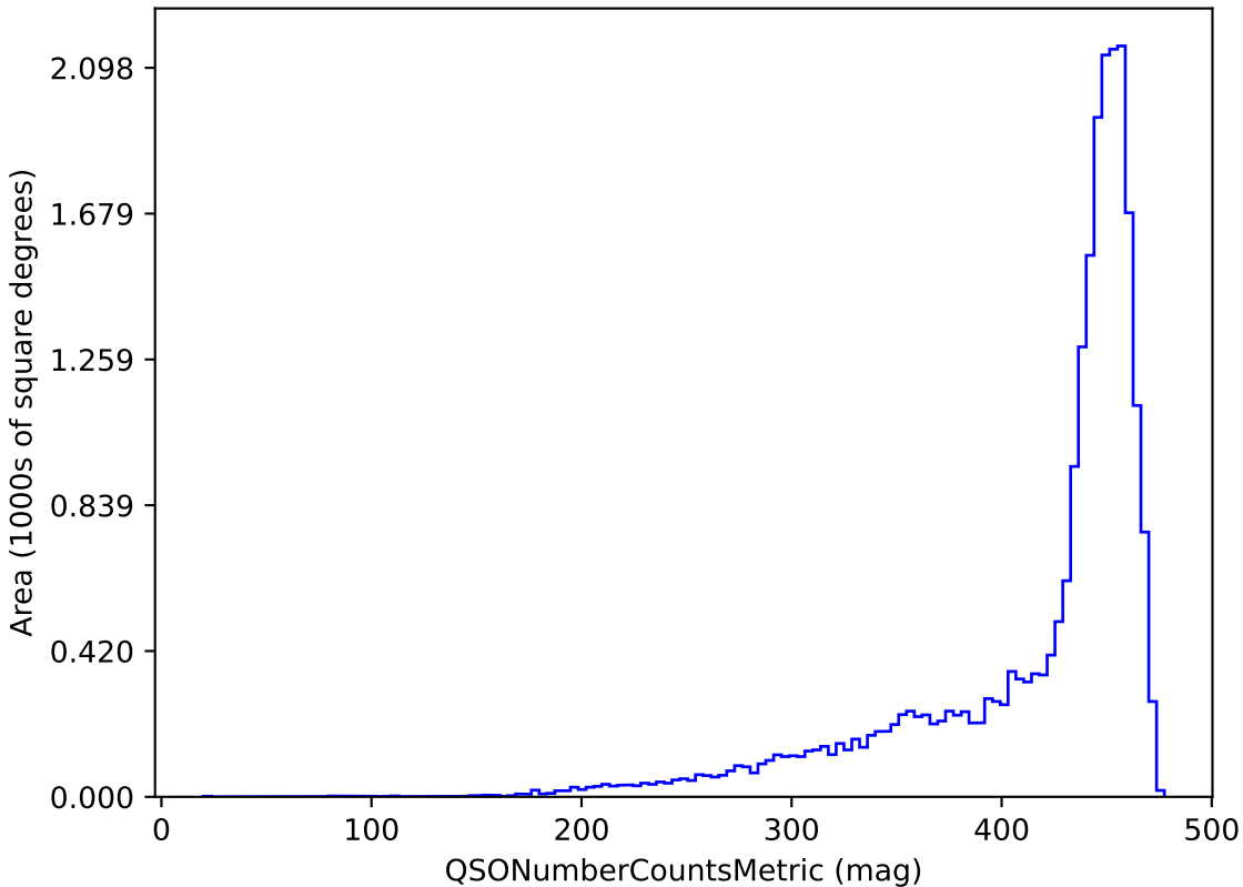
roman_v3.3_10yrs g band and non-DD: QSONumberCountsMetric
