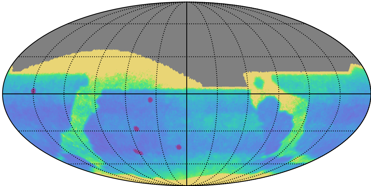
roman_v3.3_10yrs : Proper Motion Uncert @ 24.0
