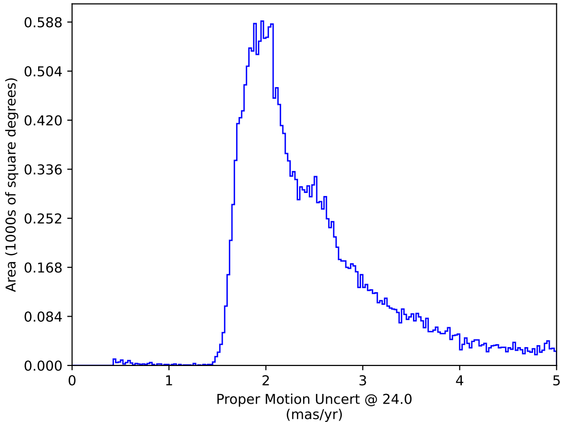
roman_v3.3_10yrs : Proper Motion Uncert @ 24.0
