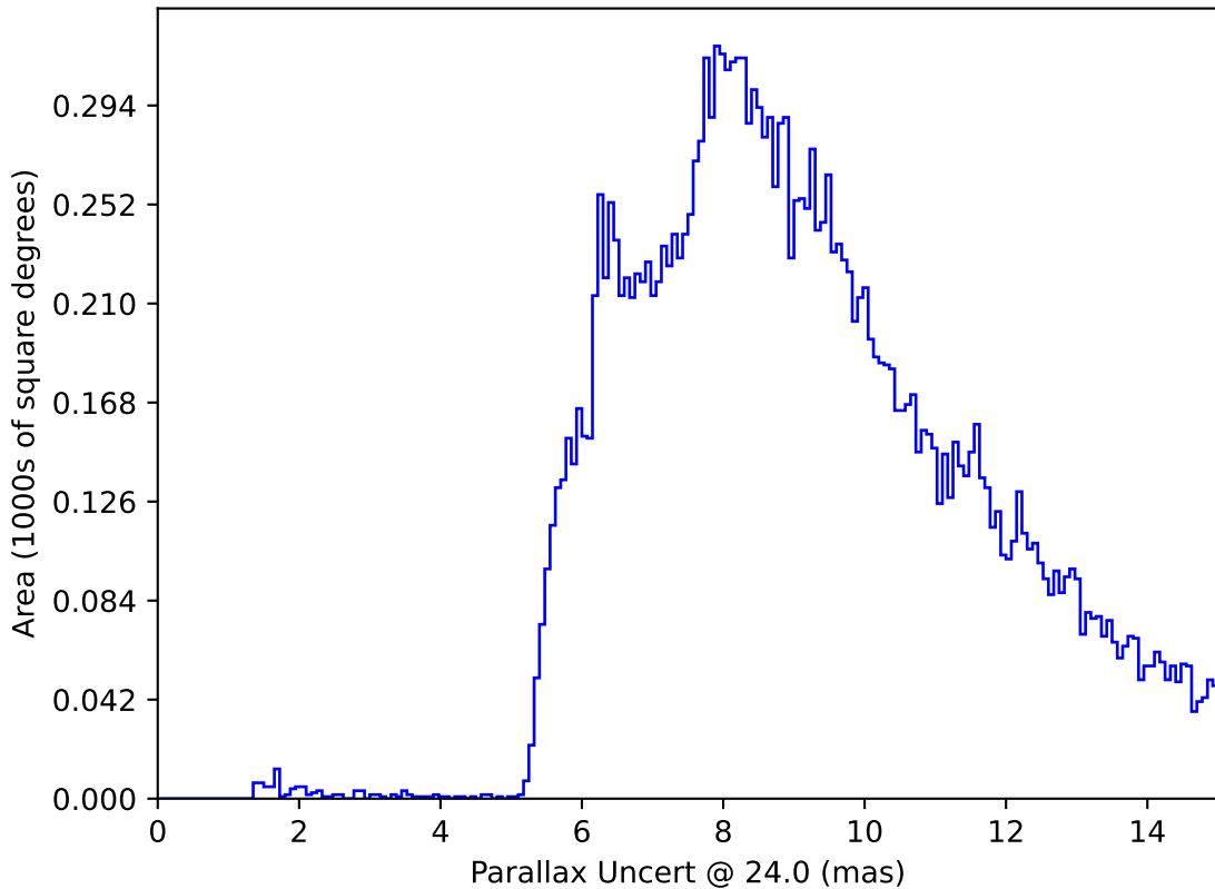
roman_v3.3_10yrs : Parallax Uncert @ 24.0
