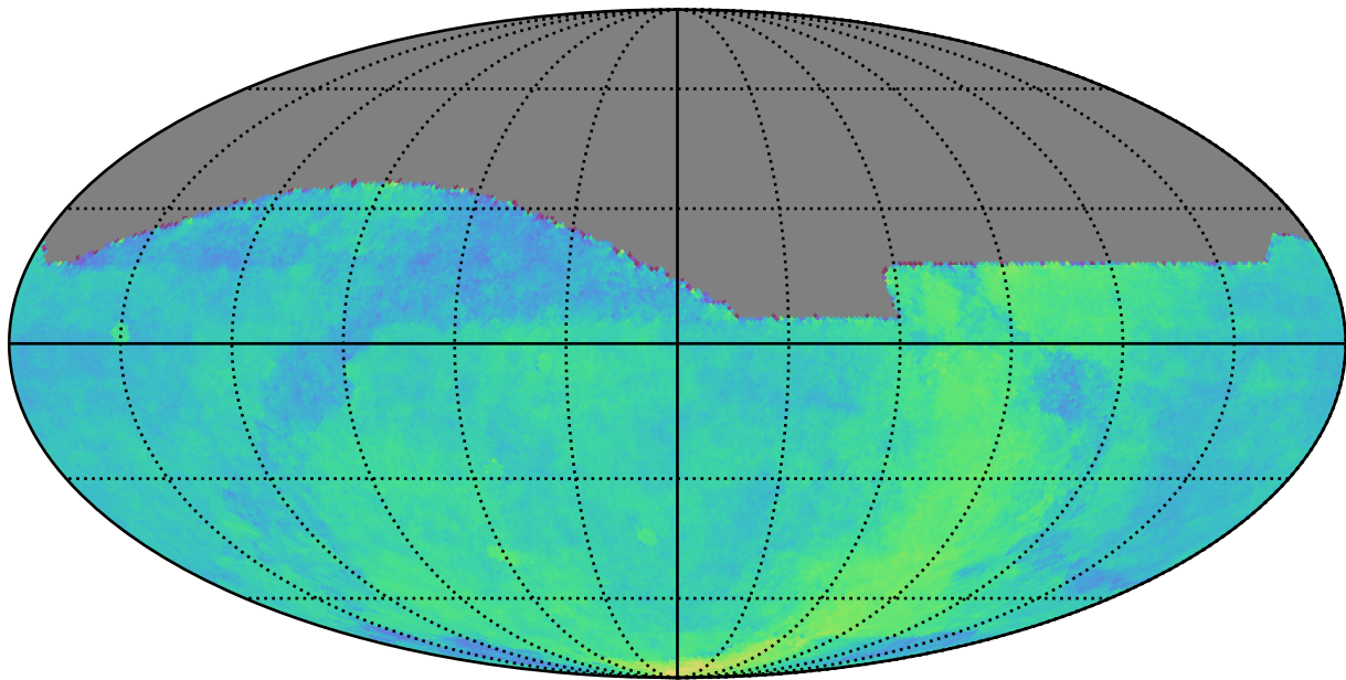
roman_v3.3_10yrs : Parallax Coverage @ 24.0
