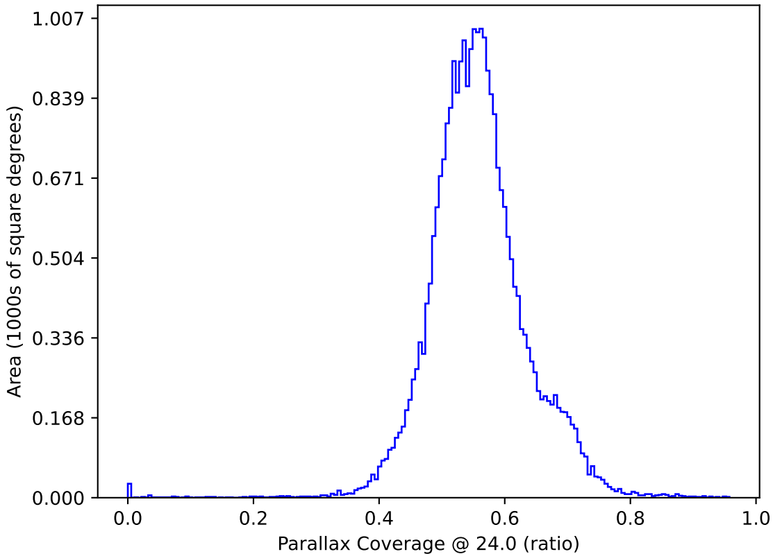
roman_v3.3_10yrs : Parallax Coverage @ 24.0
