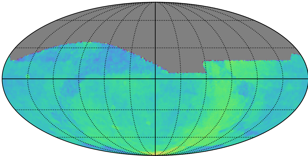
roman_v3.3_10yrs : Parallax Coverage @ 22.4
