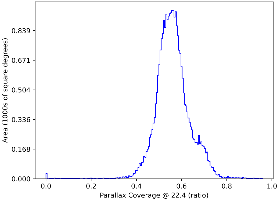
roman_v3.3_10yrs : Parallax Coverage @ 22.4
