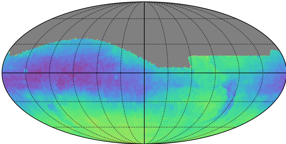
roman_v3.3_10yrs : Parallax-DCR degeneracy @ 24.0
