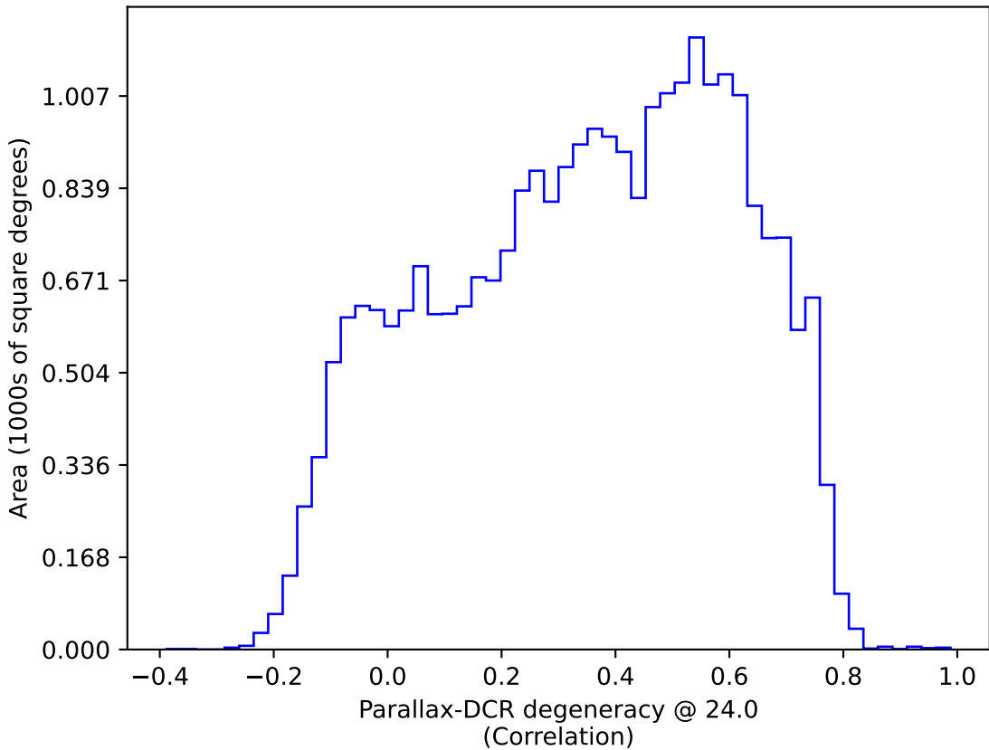
roman_v3.3_10yrs : Parallax-DCR degeneracy @ 24.0
