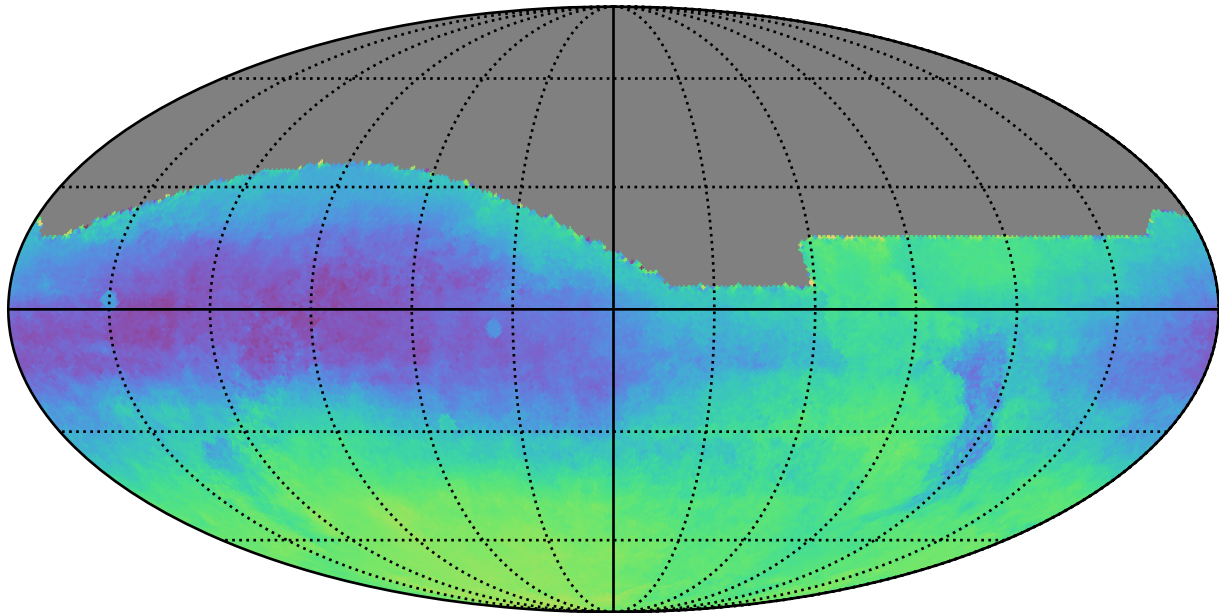
roman_v3.3_10yrs : Parallax-DCR degeneracy @ 22.4
