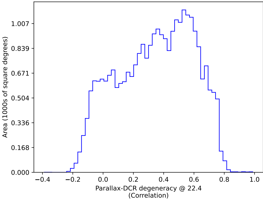
roman_v3.3_10yrs : Parallax-DCR degeneracy @ 22.4
