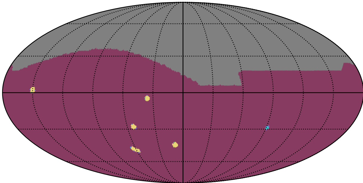
roman_v3.3_10yrs : NumberOfQuickRevisits
