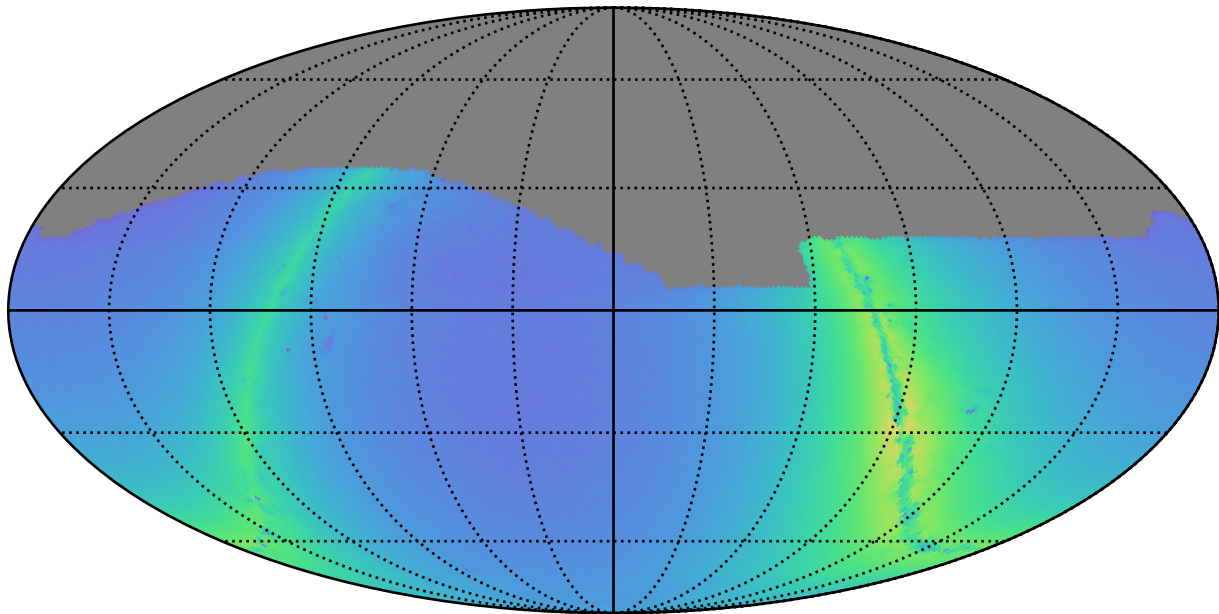
roman_v3.3_10yrs z: Nstars_no_crowding
