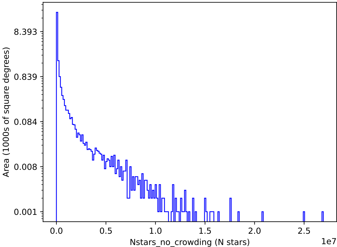
roman_v3.3_10yrs z: Nstars_no_crowding
