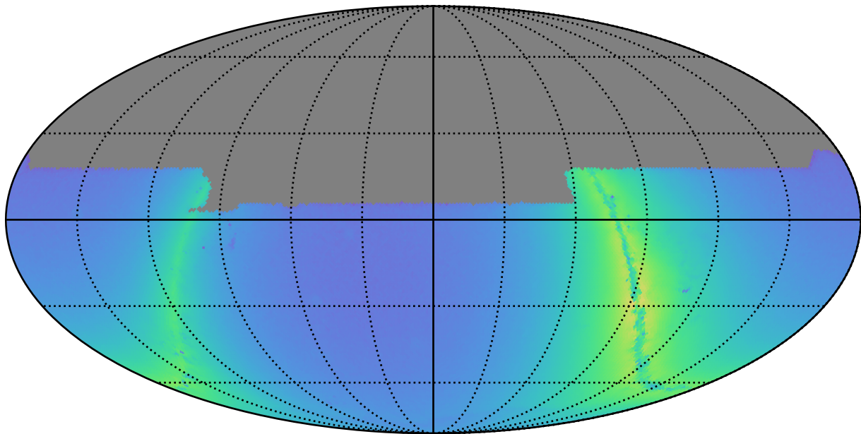
roman_v3.3_10yrs y: Nstars_no_crowding
