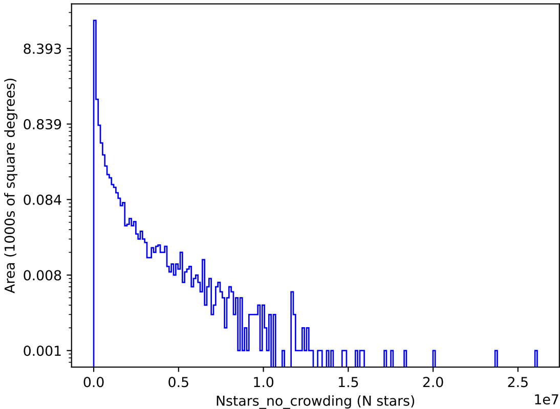
roman_v3.3_10yrs y: Nstars_no_crowding
