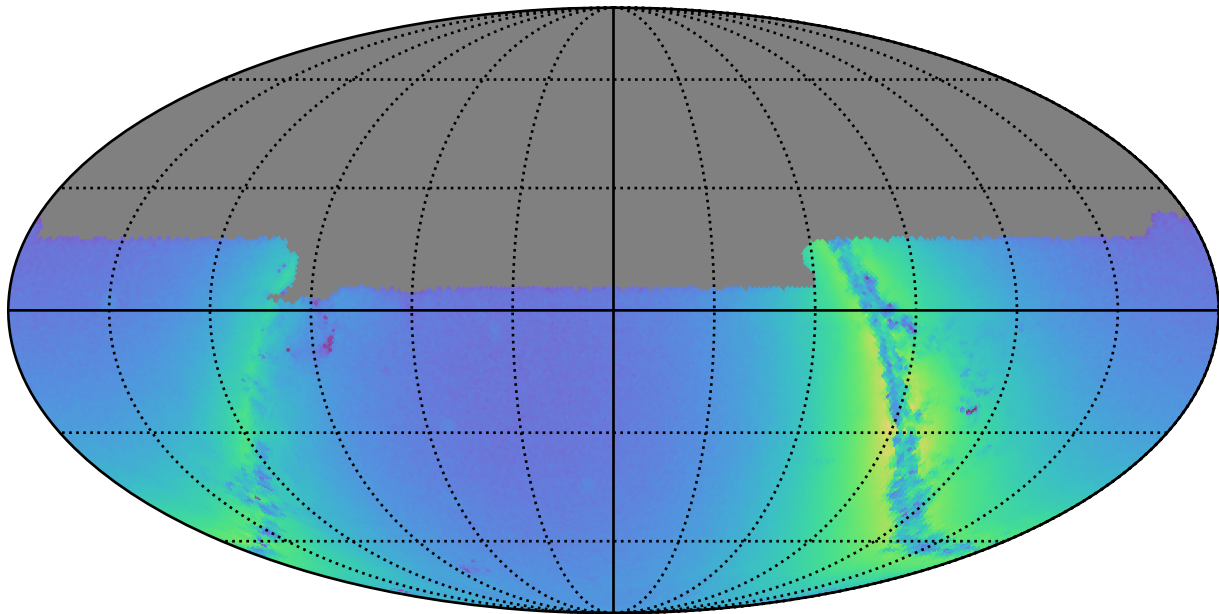
roman_v3.3_10yrs u: Nstars_no_crowding
