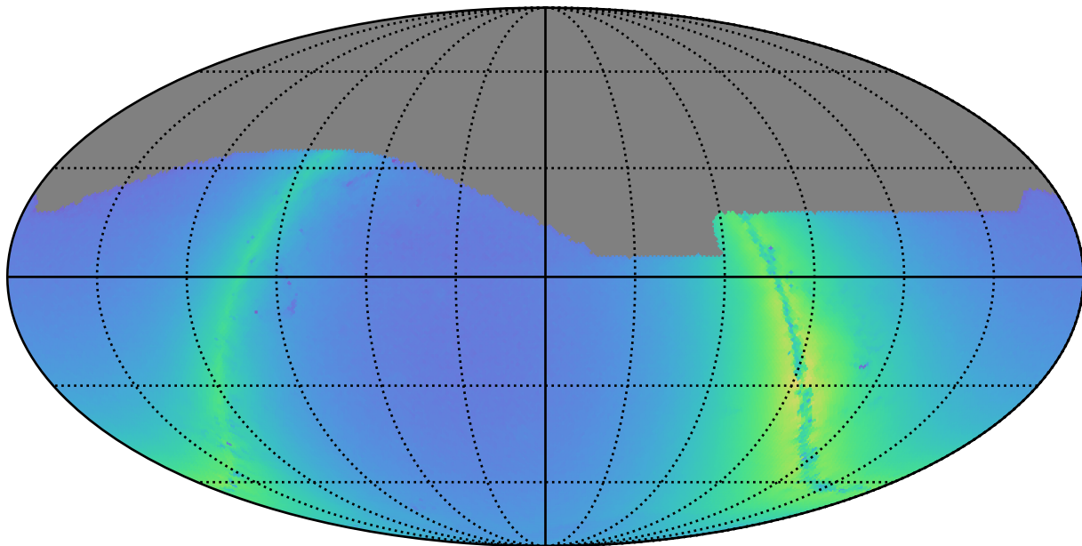
roman_v3.3_10yrs r: Nstars_no_crowding
