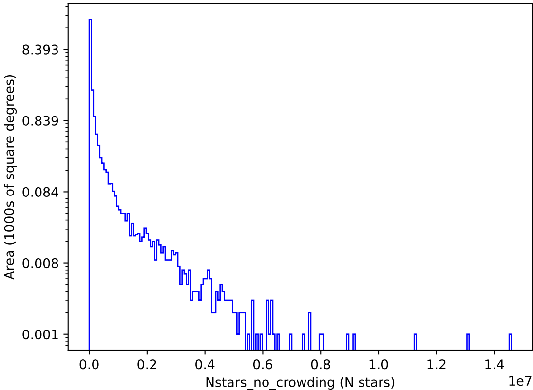
roman_v3.3_10yrs g: Nstars_no_crowding
