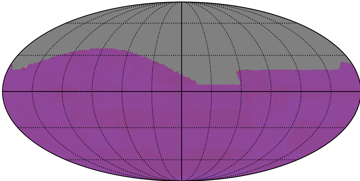
roman_v3.3_10yrs : Normalized Proper Motion Uncert @ 24.0
