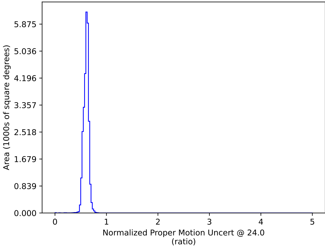
roman_v3.3_10yrs : Normalized Proper Motion Uncert @ 24.0
