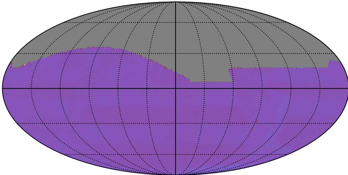
roman_v3.3_10yrs : Normalized Proper Motion Uncert @ 20.5
