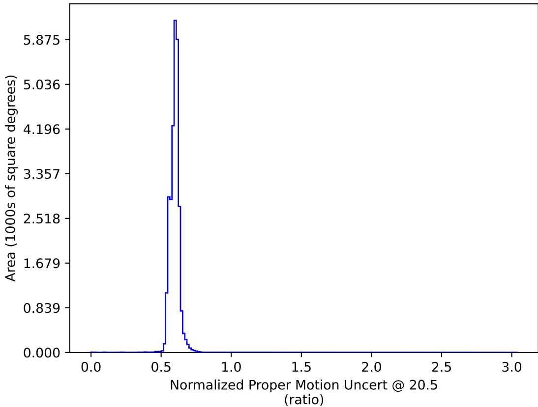
roman_v3.3_10yrs : Normalized Proper Motion Uncert @ 20.5
