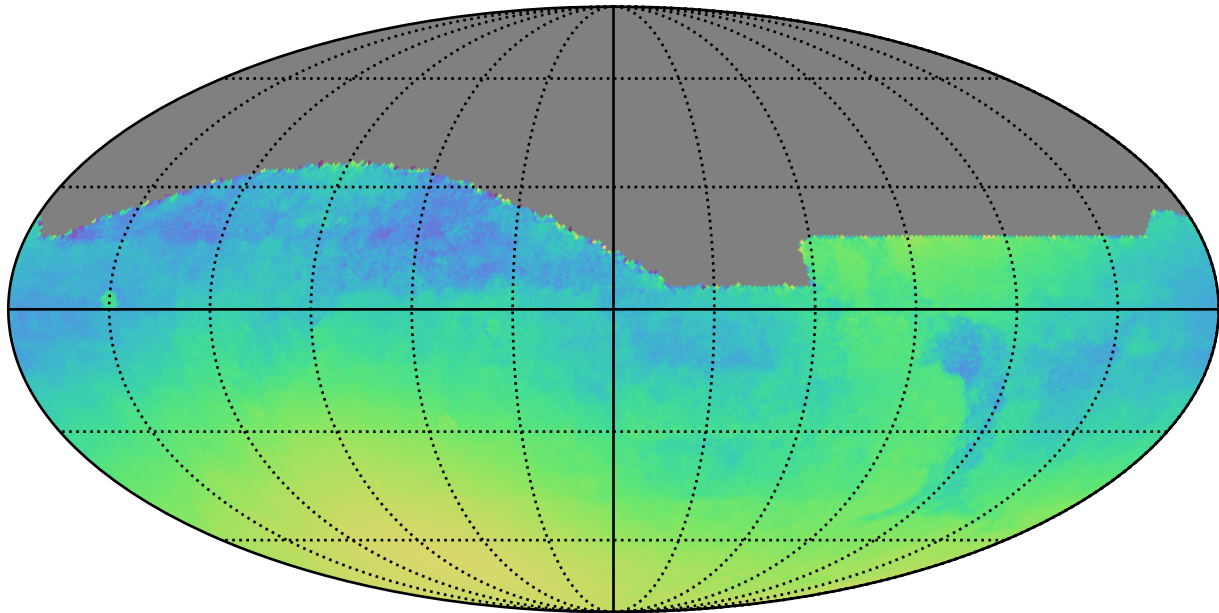
roman_v3.3_10yrs : Normalized Parallax Uncert @ 24.0
