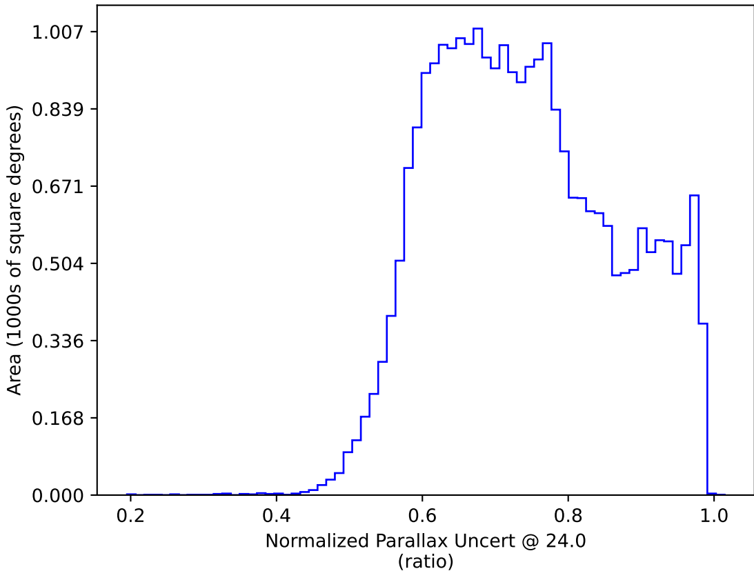
roman_v3.3_10yrs : Normalized Parallax Uncert @ 24.0
