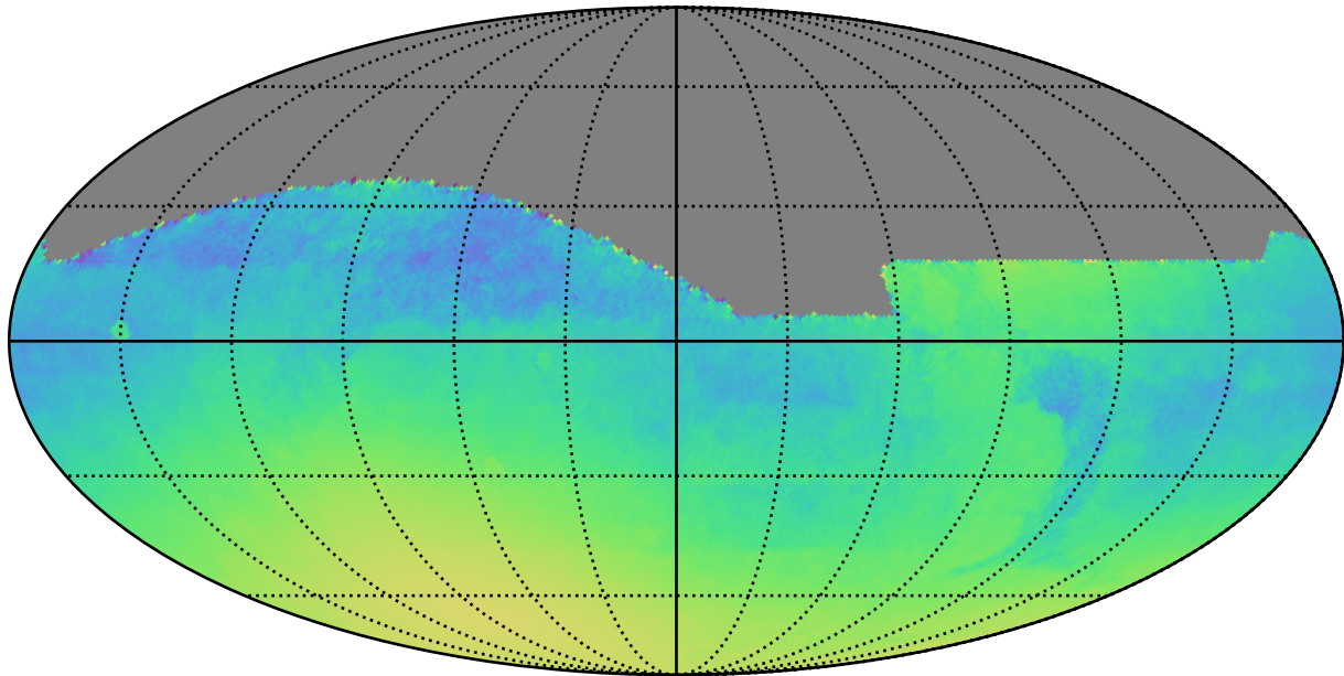
roman_v3.3_10yrs : Normalized Parallax Uncert @ 22.4
