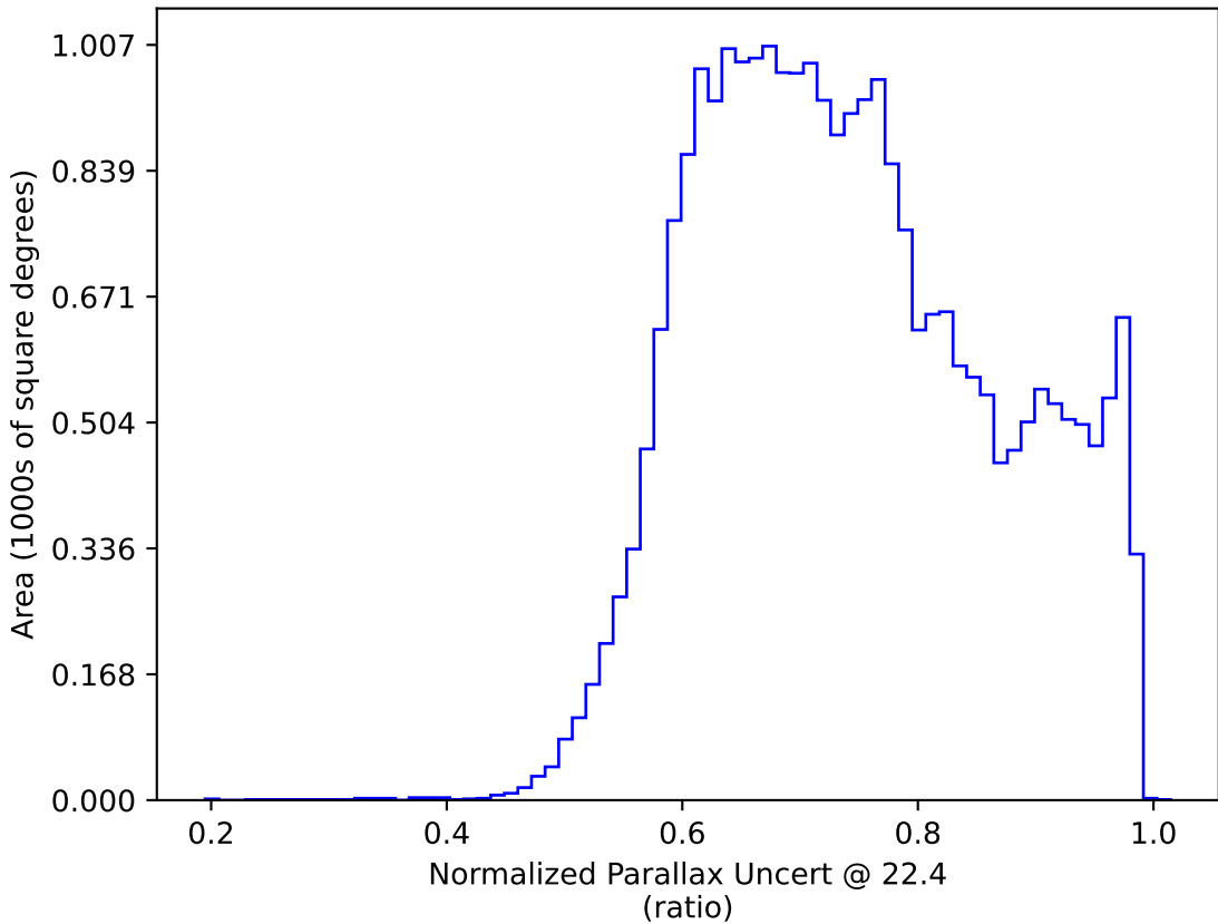
roman_v3.3_10yrs : Normalized Parallax Uncert @ 22.4
