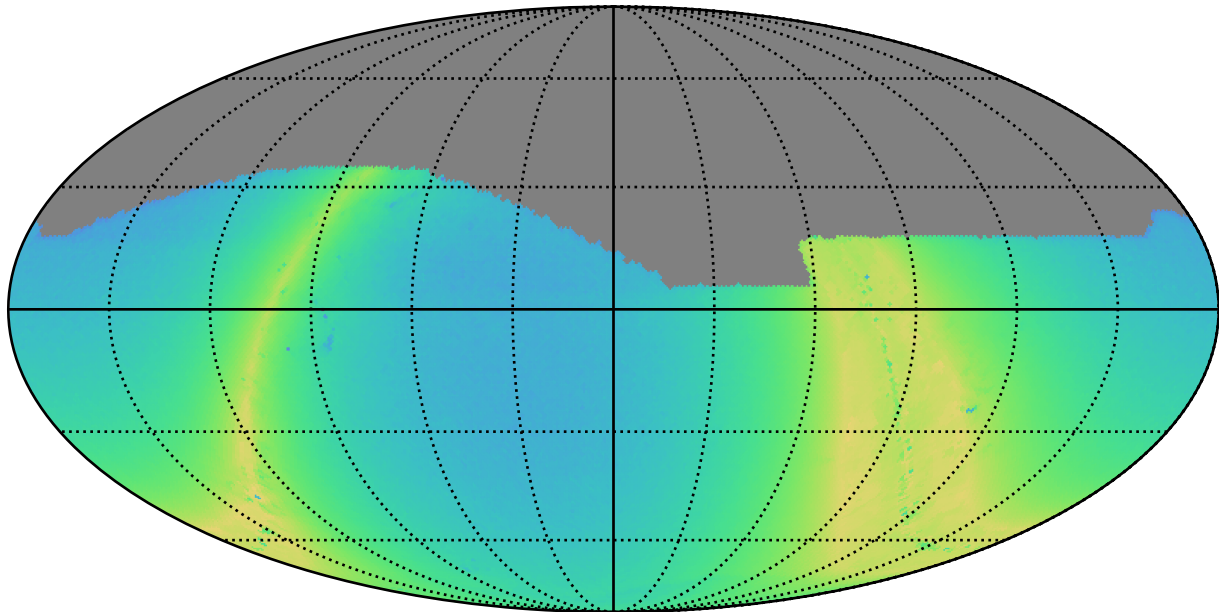
roman_v3.3_10yrs z: N stars to Precision 0.20
