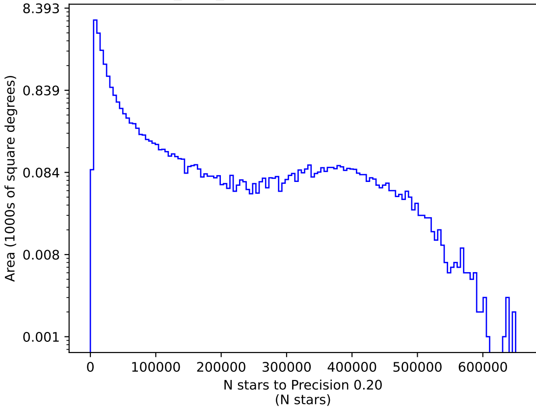
roman_v3.3_10yrs z: N stars to Precision 0.20
