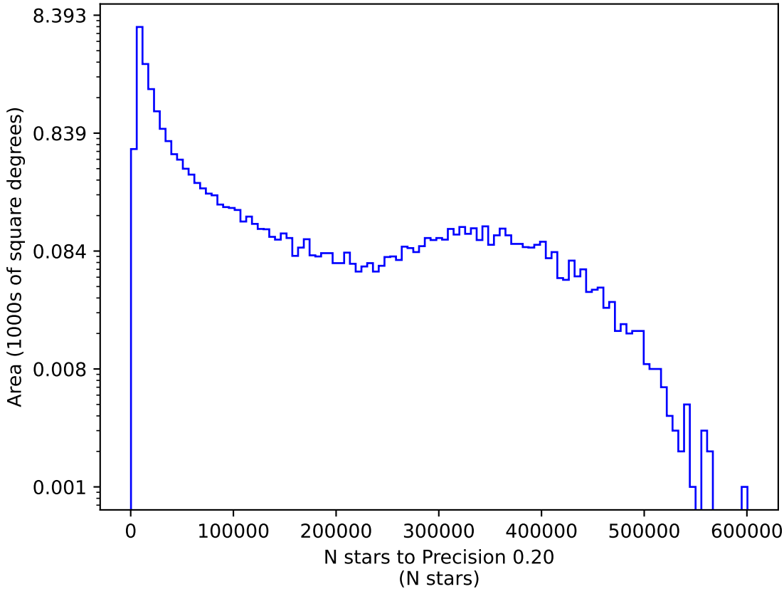
roman_v3.3_10yrs y: N stars to Precision 0.20
