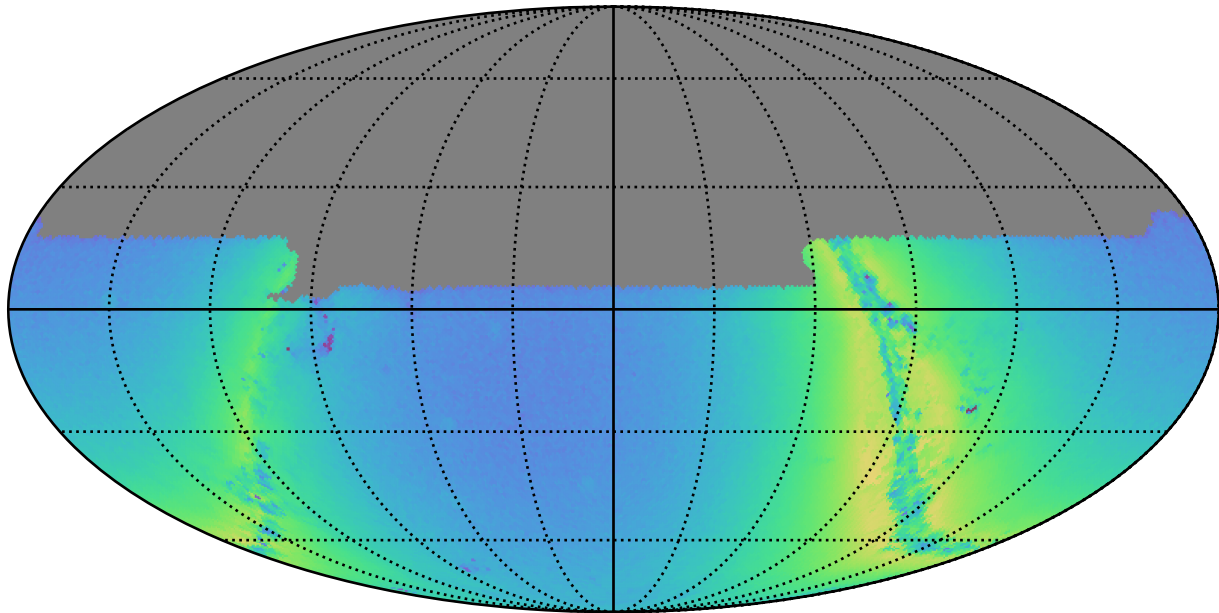
roman_v3.3_10yrs u: N stars to Precision 0.20
