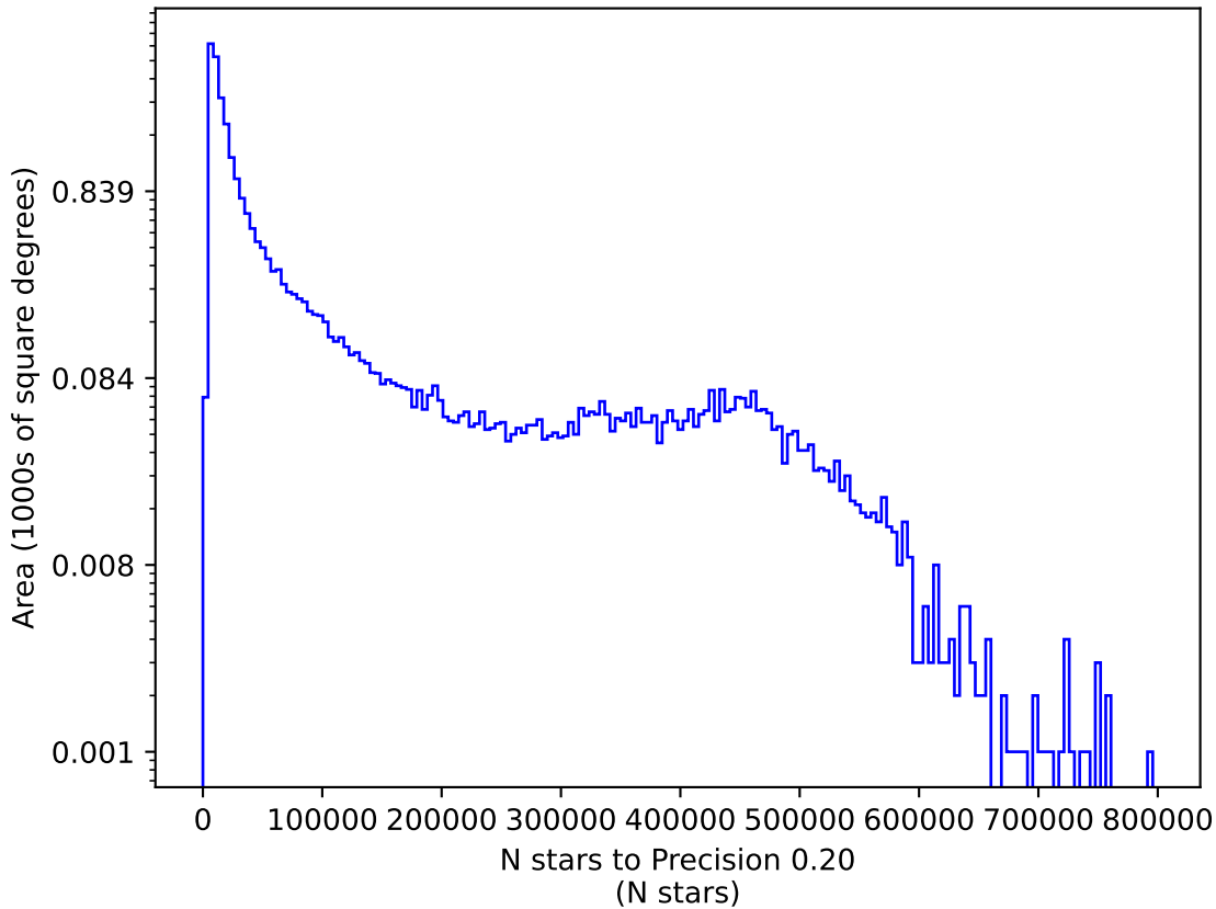
roman_v3.3_10yrs r: N stars to Precision 0.20
