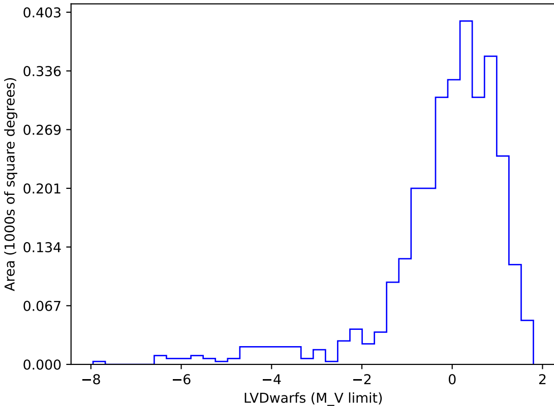
roman_v3.3_10yrs gi SCP: LVDwarfs
