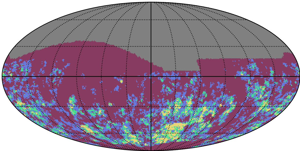
roman_v3.3_10yrs z band: Gaps_7hr
