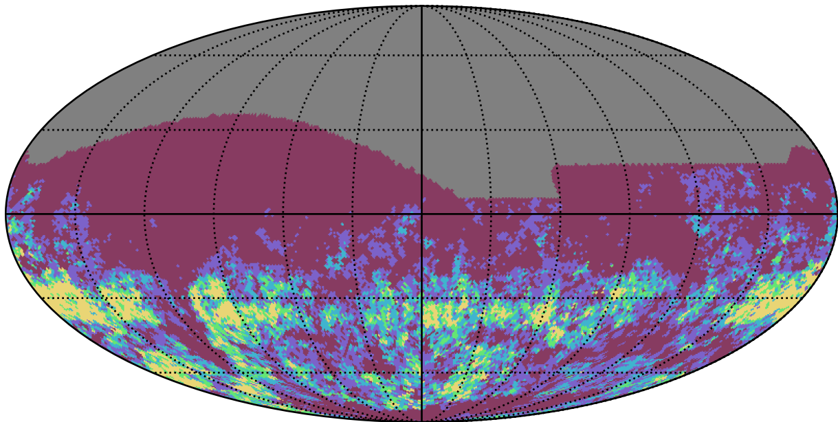
roman_v3.3_10yrs r band: Gaps_7hr
