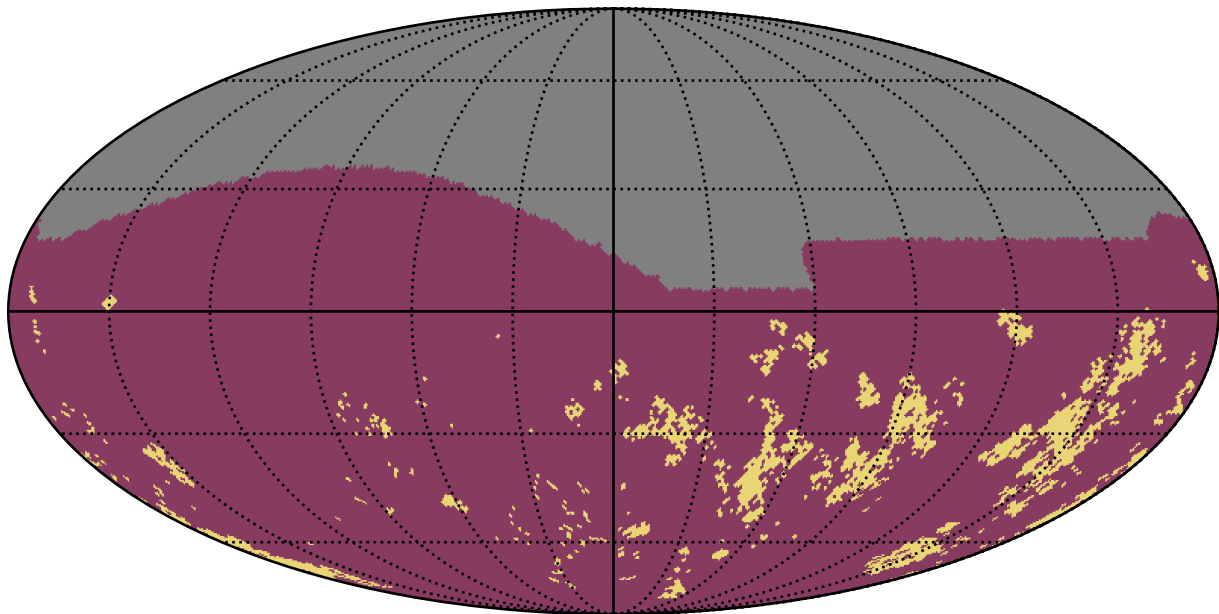
roman_v3.3_10yrs g band: Gaps_7hr
