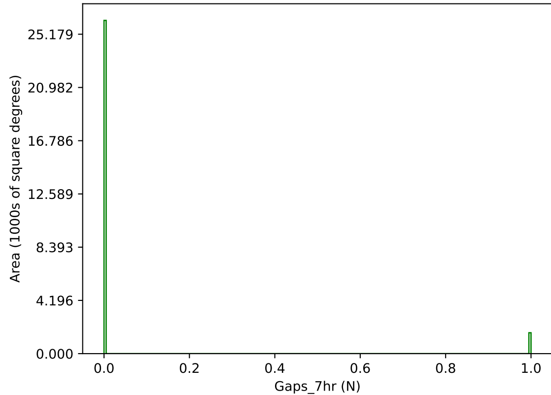
roman_v3.3_10yrs g band: Gaps_7hr
