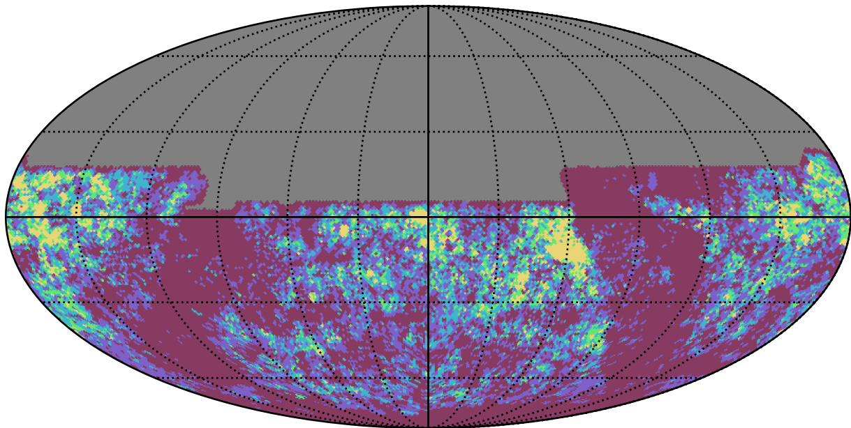
roman_v3.3_10yrs y band: Gaps_3hr
