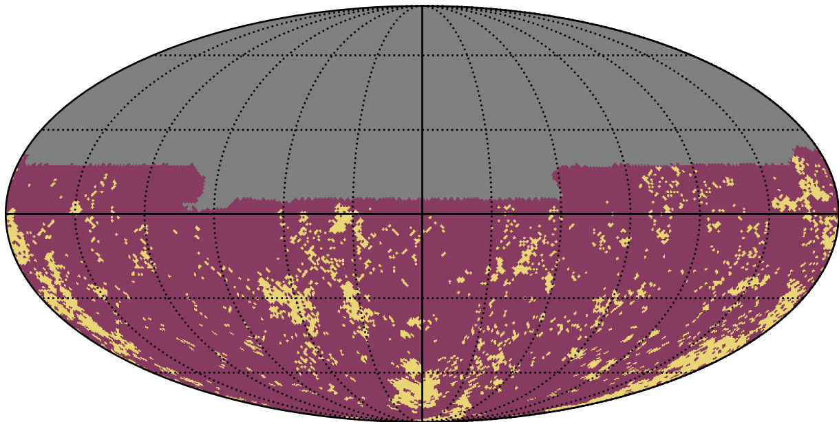
roman_v3.3_10yrs u band: Gaps_3hr
