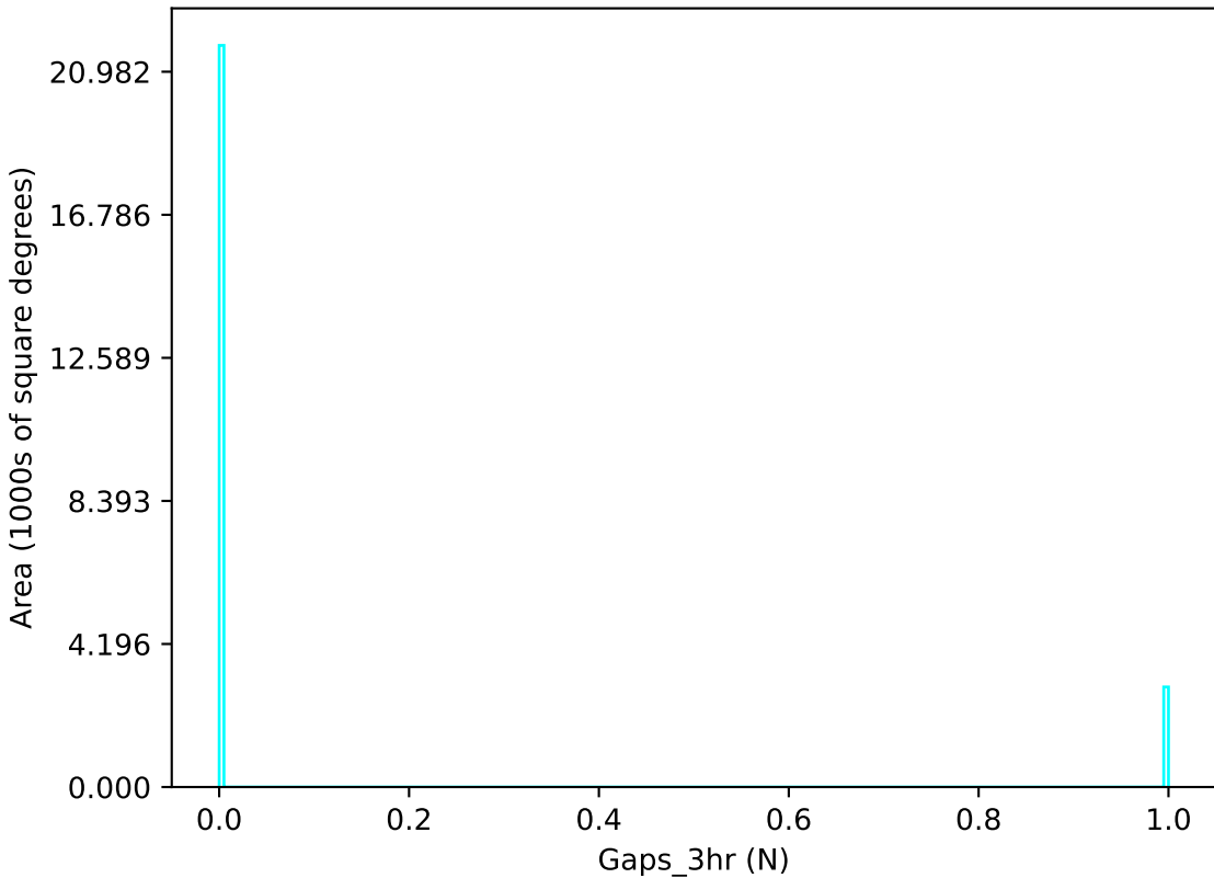
roman_v3.3_10yrs u band: Gaps_3hr
