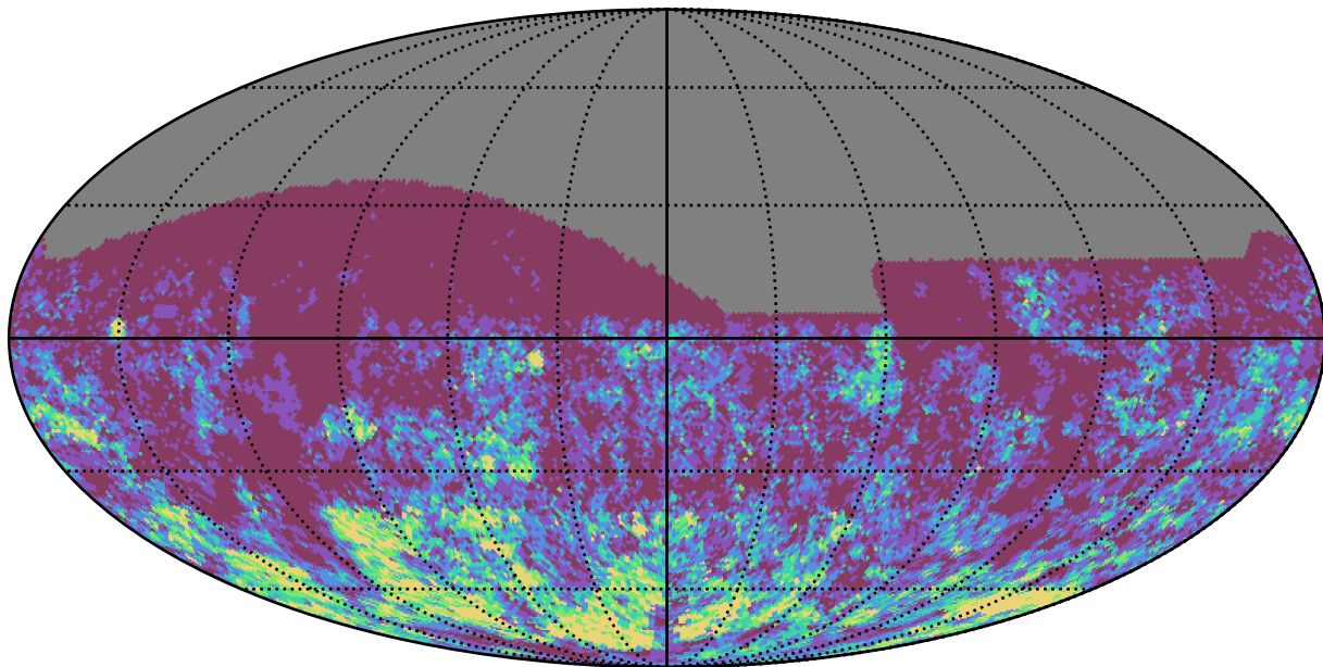
roman_v3.3_10yrs r band: Gaps_3hr
