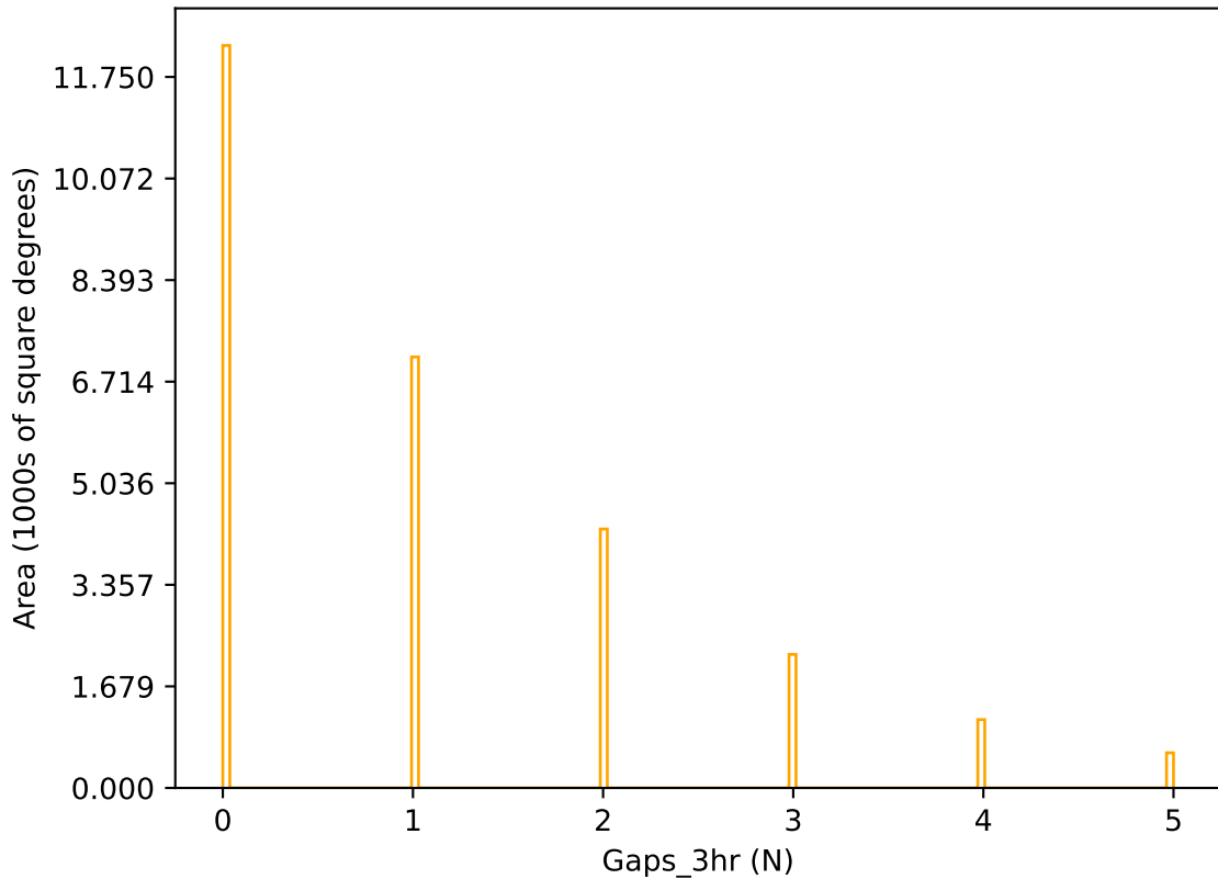
roman_v3.3_10yrs r band: Gaps_3hr
