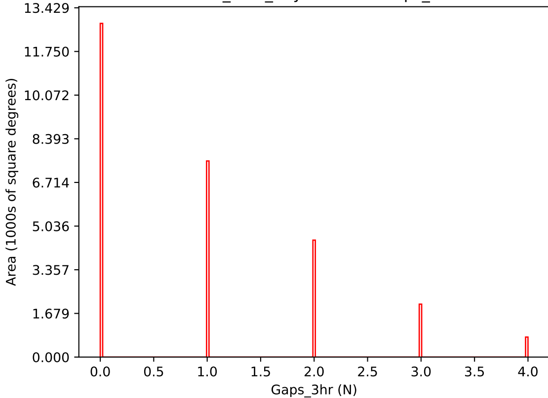
roman_v3.3_10yrs i band: Gaps_3hr
