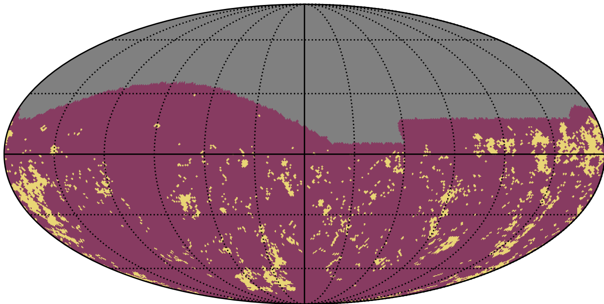
roman_v3.3_10yrs g band: Gaps_3hr
