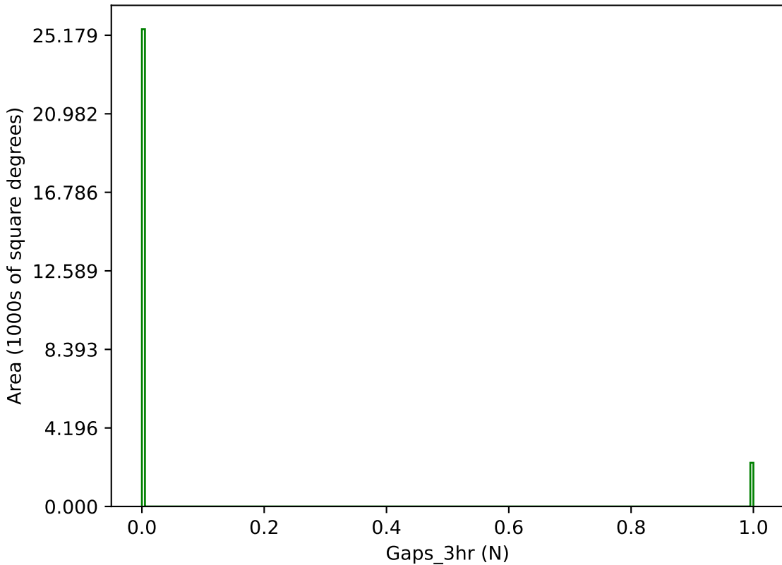
roman_v3.3_10yrs g band: Gaps_3hr
