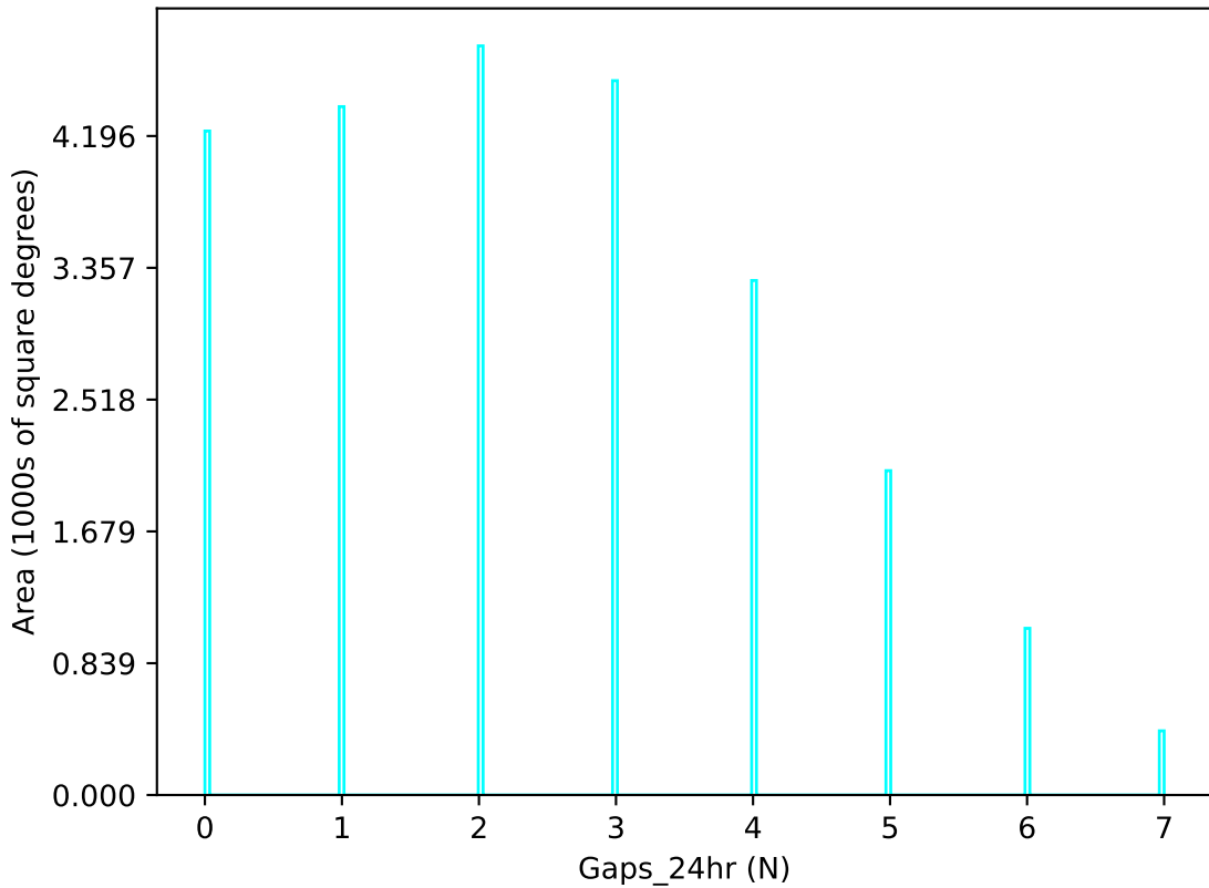
roman_v3.3_10yrs u band: Gaps_24hr
