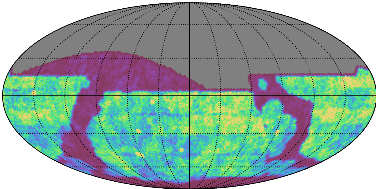
roman_v3.3_10yrs r band: Gaps_24hr
