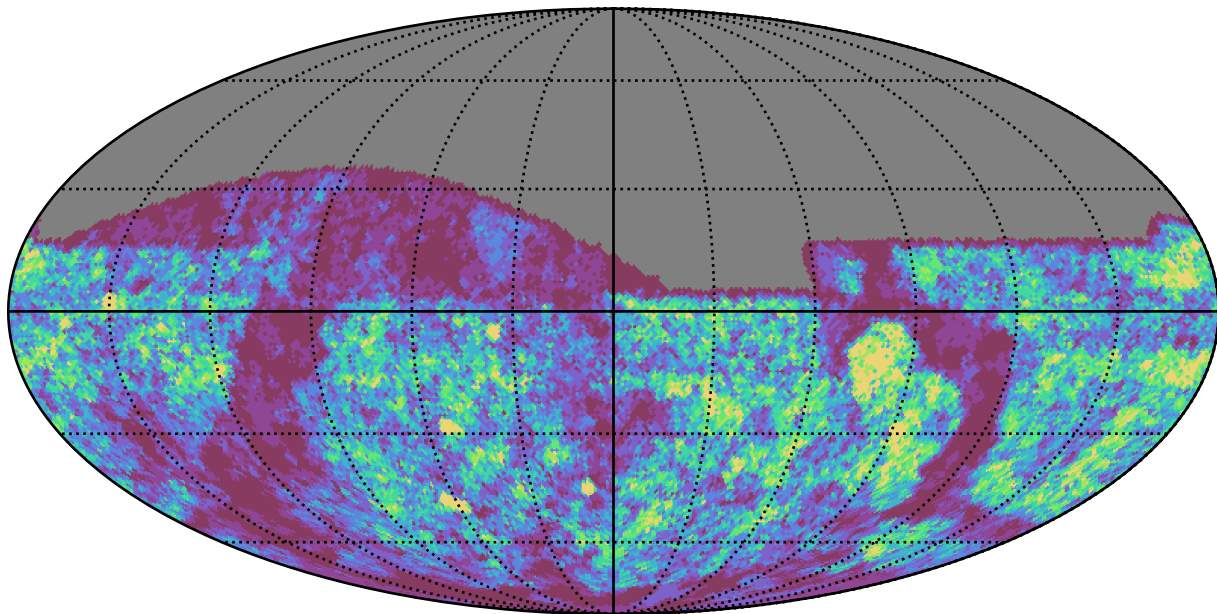
roman_v3.3_10yrs g band: Gaps_24hr
